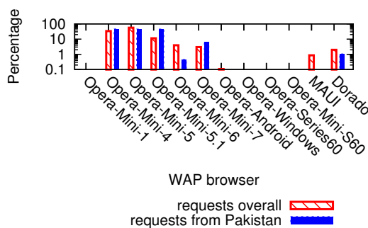
Figure 10: Proportion of WAP browsers
