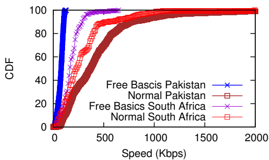
Figure 3: CDF of page fetch speeds
