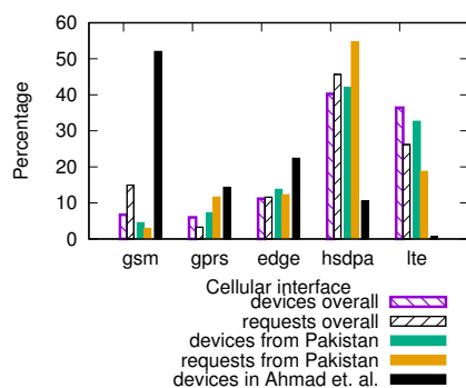
Figure 12: Proportion of cellular interfaces
