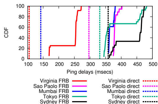
Figure 6: Ping delays for different web server locations for SA client.
