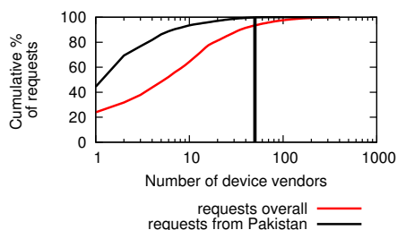
Figure 9: Devices from 50 vendors send 90% of requests.
